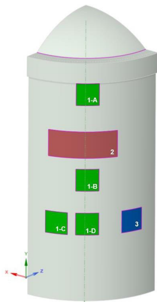
Figure 3: ANSYS 1/4 Model of a Containment Structure
