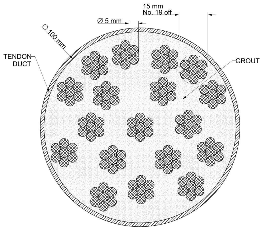
Figure 4: Schematic of Tendon Cross Section
